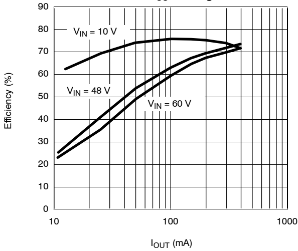
Output Load vs. Efficiency (Si9121DY-3) With V CC Winding
